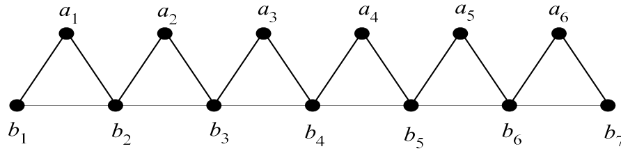
Figure 1: Triangular snake graph T_7 .
