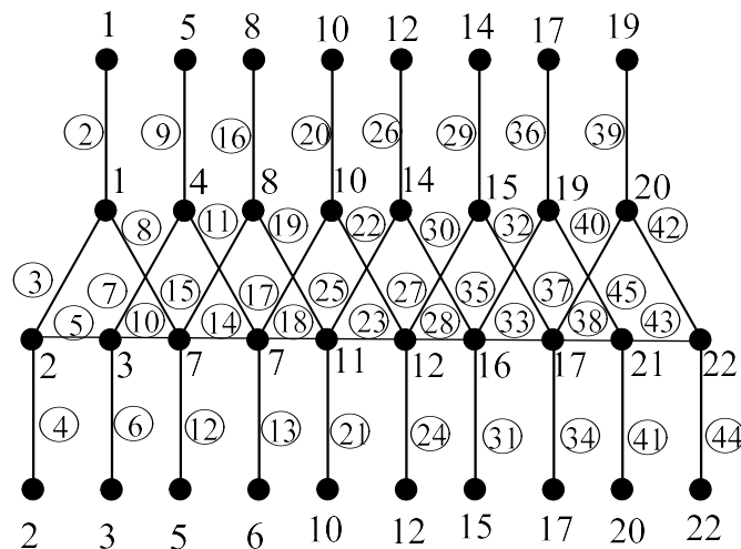
Figure 8: Irregular labeling on alternate triangular snake graph AT_{10} with pendant edges.
