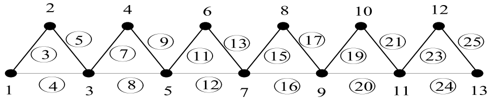
Figure 5: Irregular labeling on triangular snake graph T_7 .
