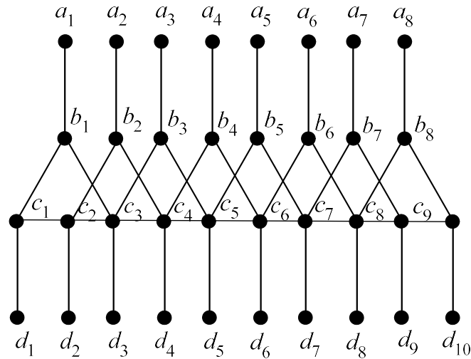
Figure 4: Alternate triangular snake graph AT_{10} with pendant edges.
