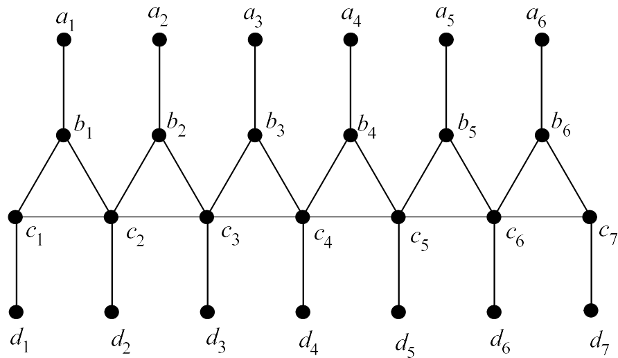
Figure 2: Triangular snake graph T_7 with pendant edges.
