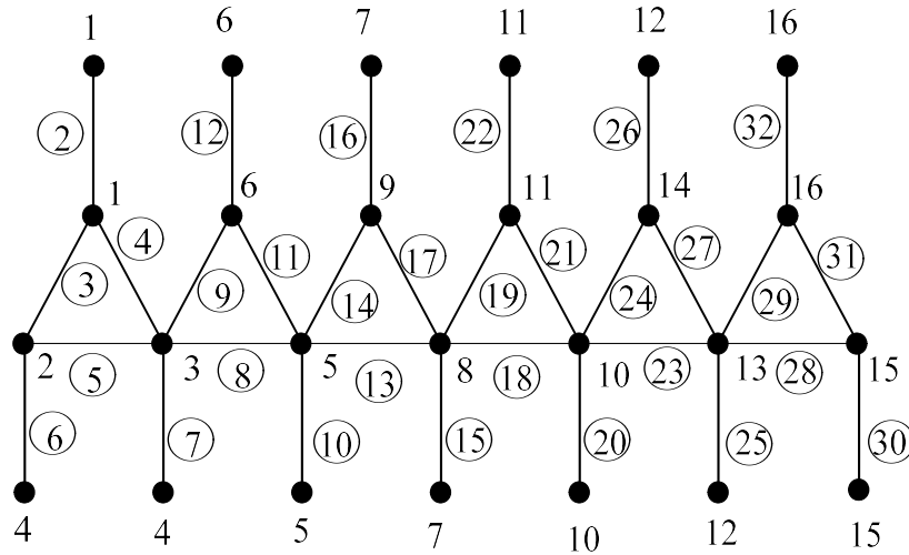
Figure 6: Irregular labeling on triangular snake graph T_7 with pendant edges.
