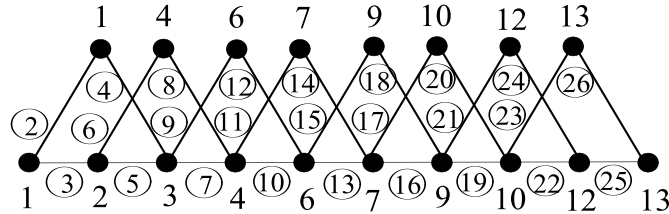
Figure 7: Irregular labeling on alternate triangular snake graph AT_{10} .
