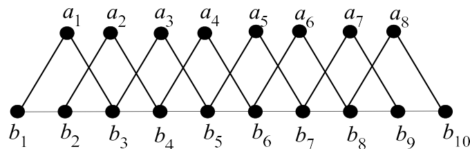
Figure 3: Alternate triangular snake graph AT_{10} .
